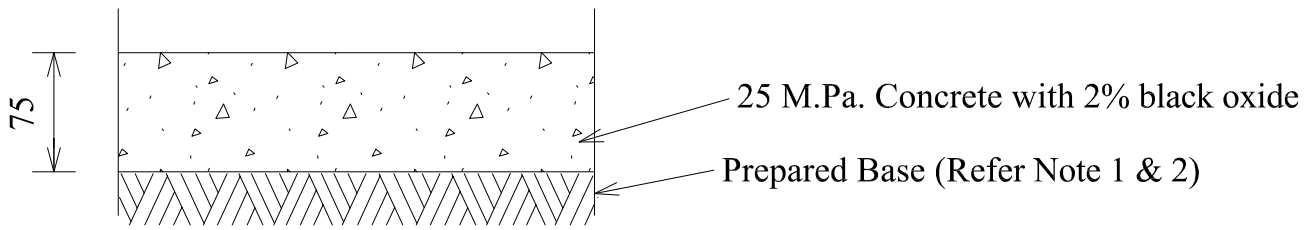
CONCRETE FOOTPATH
