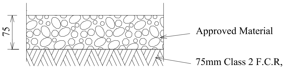
GRANITIC FOOTPATH
