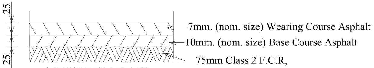
ASPHALT FOOTPATH
