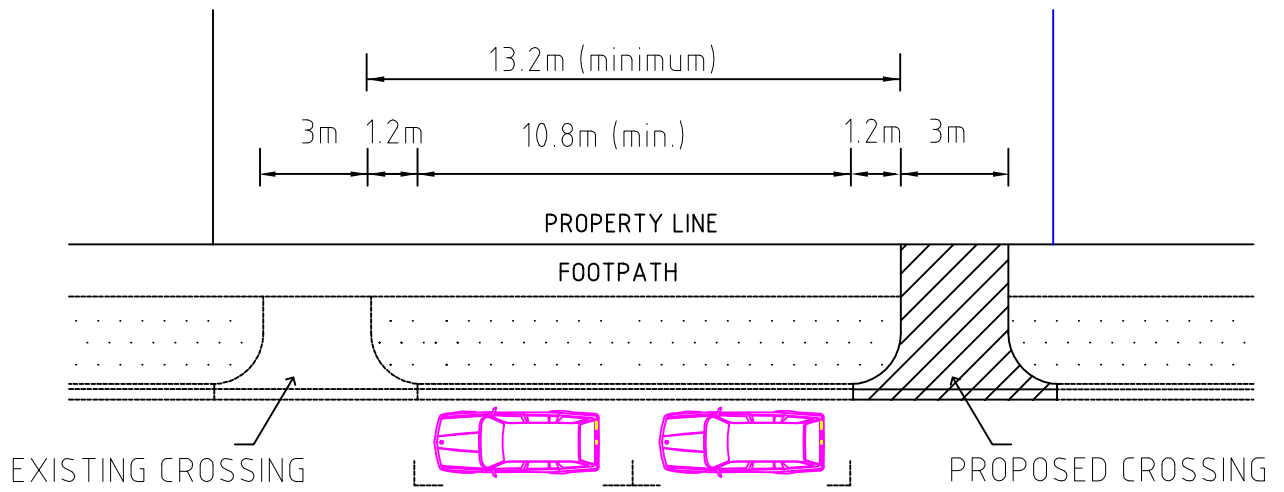
DIAGRAM 1 - MINIMUM DIMENSIONS FOR SECOND CROSSINGS
