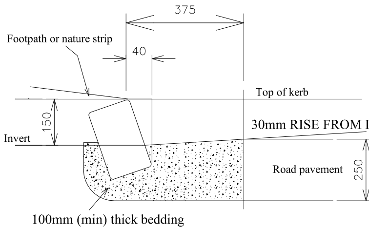
BLUESTONE KERB AND CONCRETE CHANNEL
