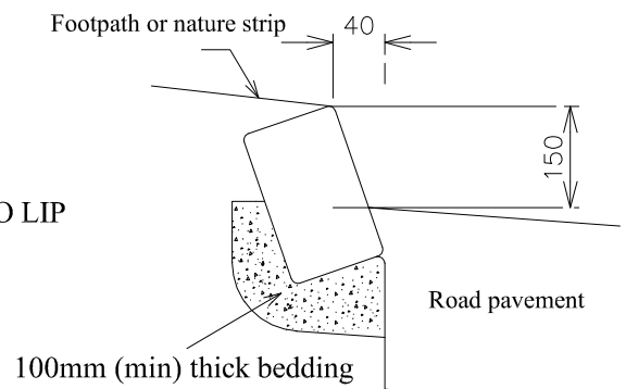
BLUESTONE KERB (NO CHANNEL)
