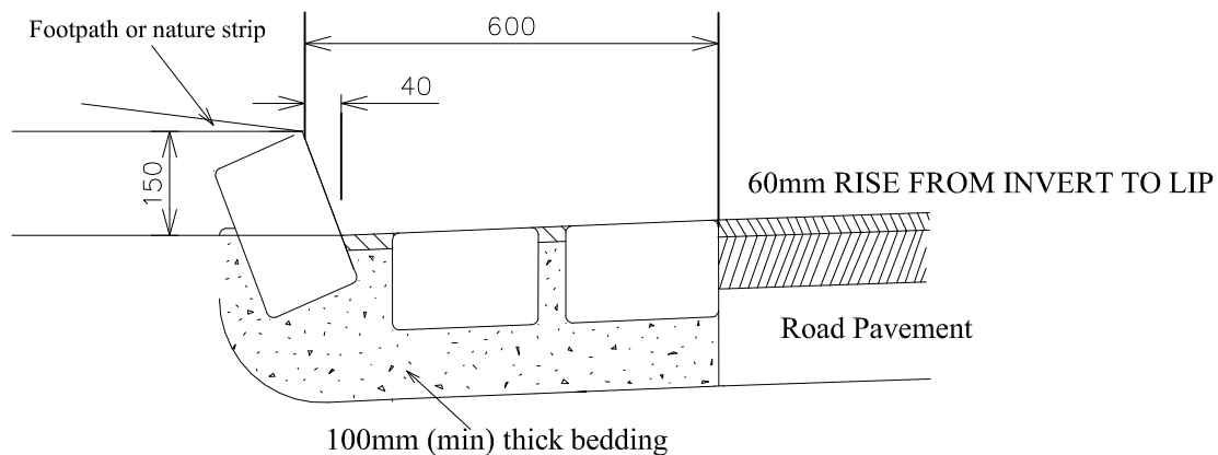
BLUESTONE KERB AND TWO BLUESTONE CHANNEL
