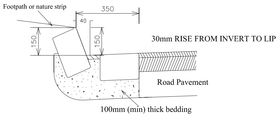
BLUESTONE KERB AND CONCRETE CHANNEL
